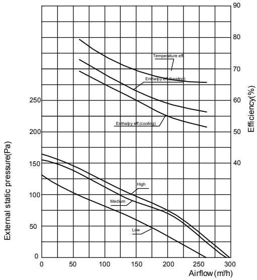
CH-HRV2K2 Performance Chart
