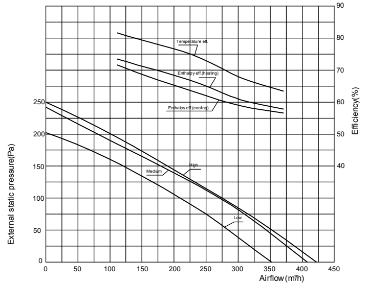
CH-HRV3K2 Performance Chart
