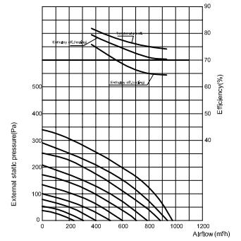
CH-HRV8KDC Performance Chart
