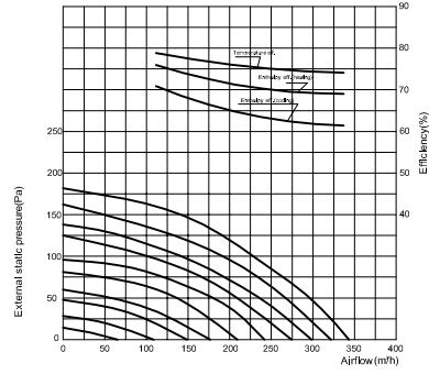
CH-HRV2.5KDC Performance Chart
