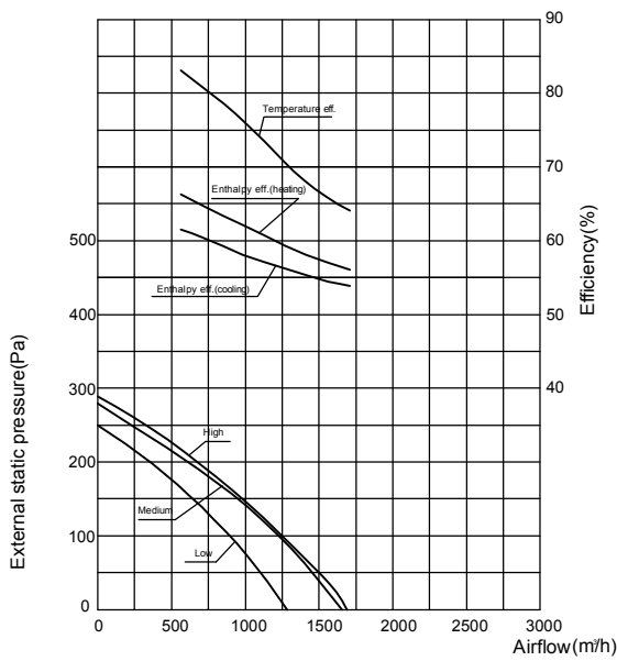
CH-HRV13K2 Performance Chart
