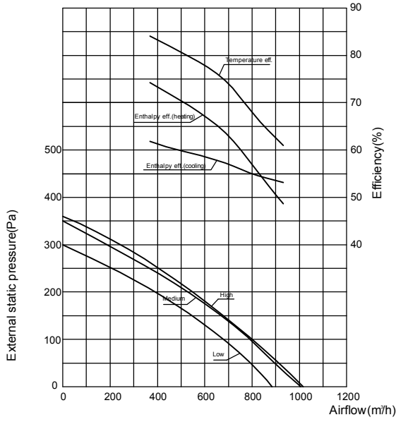
CH-HRV8K2 Performance Chart
