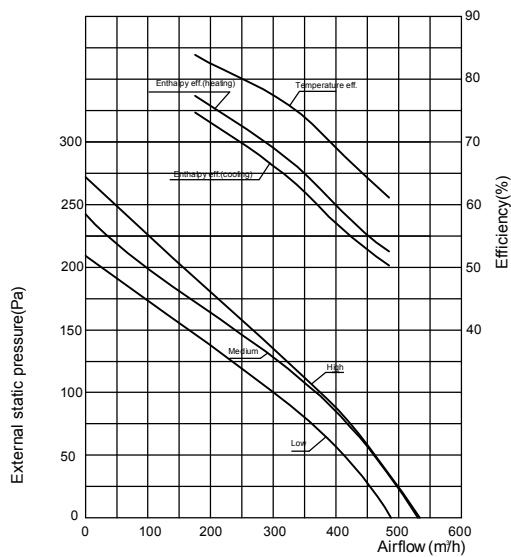
CH-HRV4K2 Performance Chart
