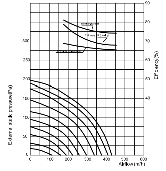
CH-HRV3.5KDC Performance Chart
