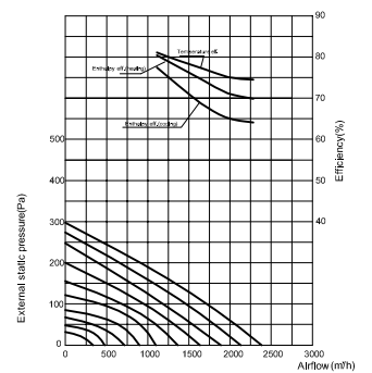
CH-HRV20KDC Performance Chart
