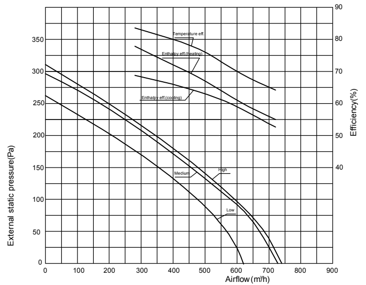
CH-HRV6K2 Performance Chart
