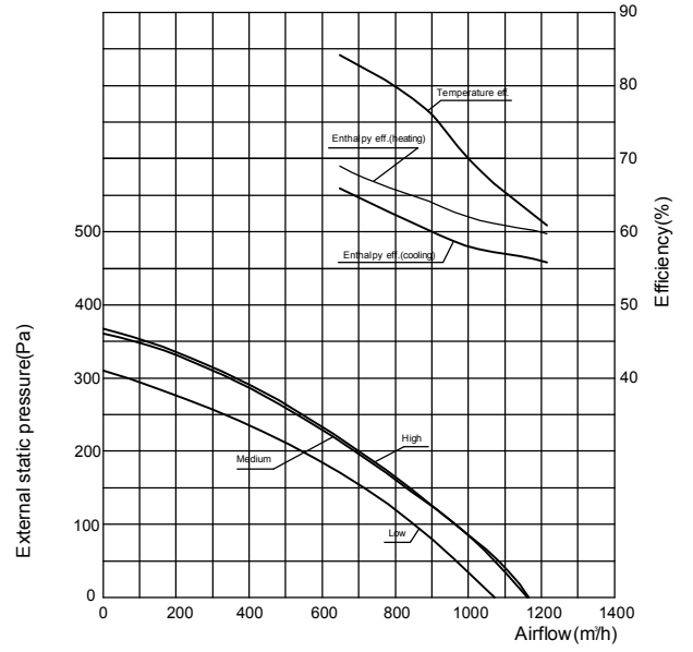
CH-HRV10K2 Performance Chart
